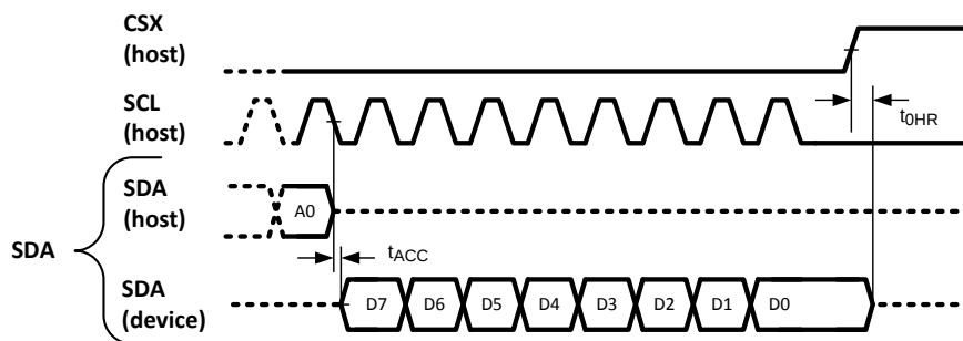
Figure 5. SPI Interface
